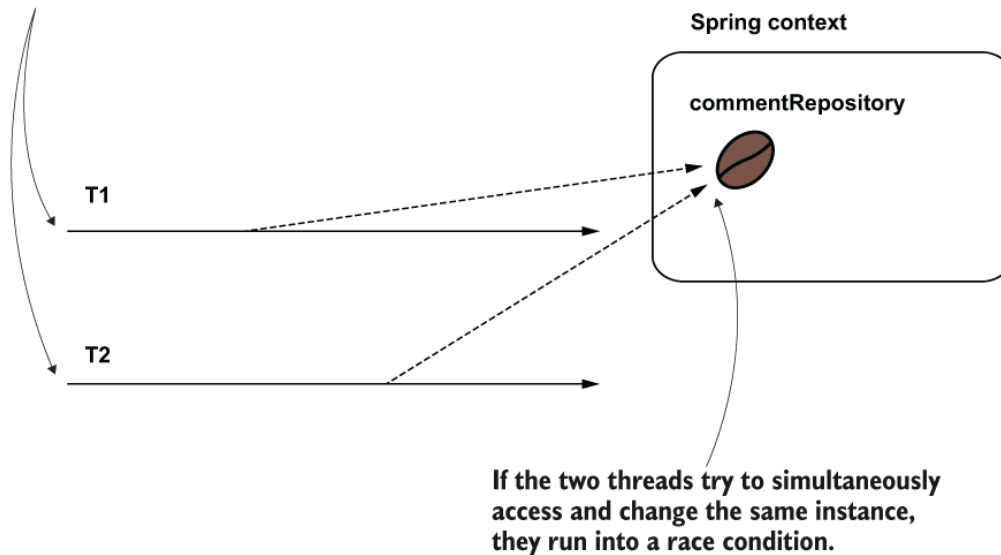
Figure 5.5 When multiple threads access a singleton bean, they access the same instance. If these threads try to change the instance simultaneously, they run into a race condition. The race condition causes unexpected results or execution exceptions if the bean is not designed for concurrency.
