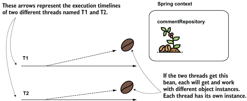
Figure 5.7 When multiple threads request a certain prototype bean, each thread gets a different instance. This way, the threads cannot run into a race condition.
