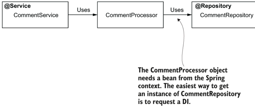
Figure 5.10 If the CommentProcessor object needs to use an instance of CommentRepository , the easiest way to get an instance is to request a DI. But to do this, Spring needs to know about CommentProcessor , so the CommentProcessor object needs to be a bean in the context.
