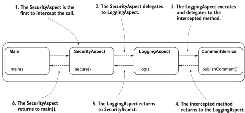
Figure 6.16 The execution flow after changing the order of the aspects. The SecurityAspect was first to intercept the method call and delegates further in the execution chain to the LoggingAspect, which further delegates the call to the intercepted method. The intercepted method returns to the LoggingAspect, which returns further to the SecurityAspect.
