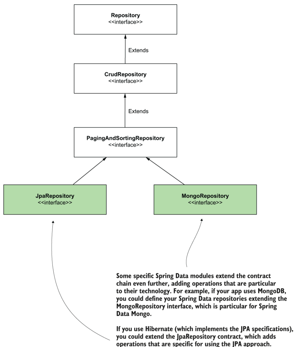
Figure 14.9 Spring Data modules that are specific to certain technologies might provide particular contracts that define operations you can apply only with those technologies. When using such technologies, your app most likely will use these specific contracts.
