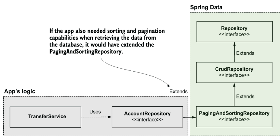
Figure 14.8 If the app needs sorting and paging capabilities, it should extend a more particular contract. The app provides a bean that implements the contract, which can then be injected from any other component that needs to use it.
