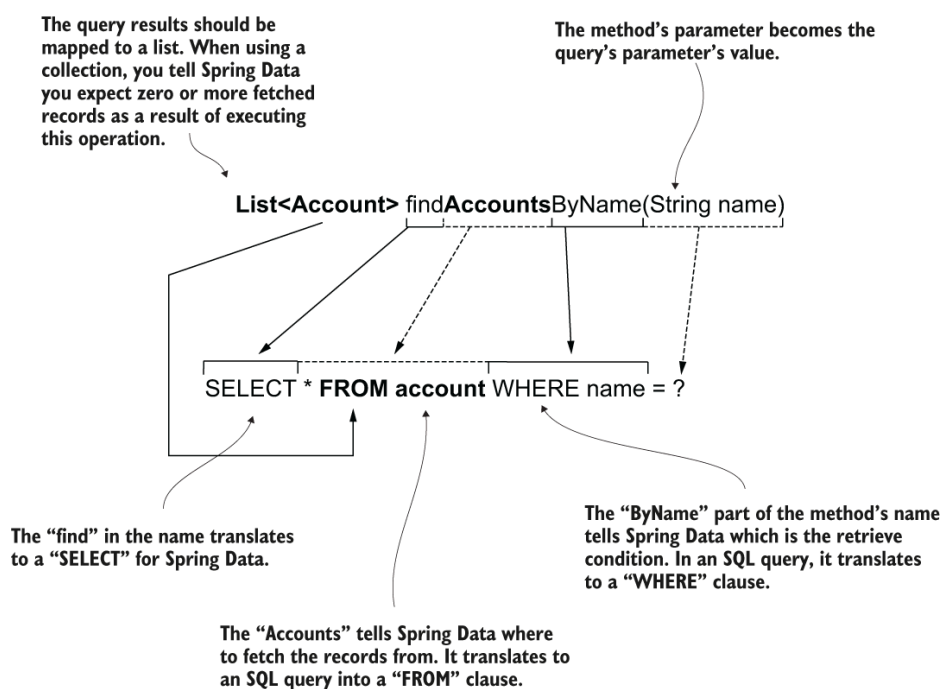
Figure 14.12 The relationship between the repository's method name and the query Spring Data creates behind the scenes
