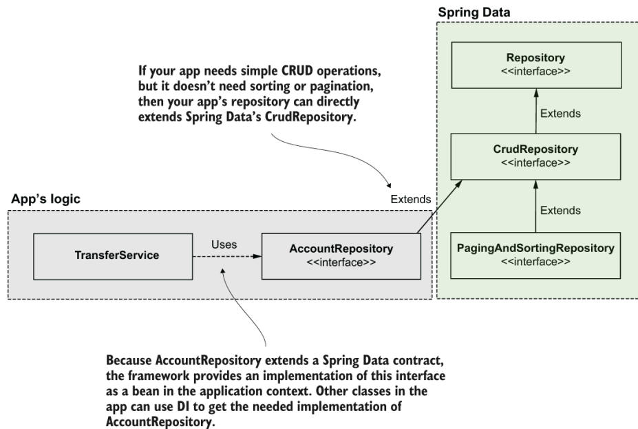
Figure 14.7 To create a Spring Data repository, you define an interface that extends one of the Spring Data contracts. For example, if your app only needs CRUD operations, the interface you define as a repository should extend the CrudRepository interface. The app adds a bean that implements the contract you define to the Spring context, so any other app components that need to use it can simply inject it from the context.
