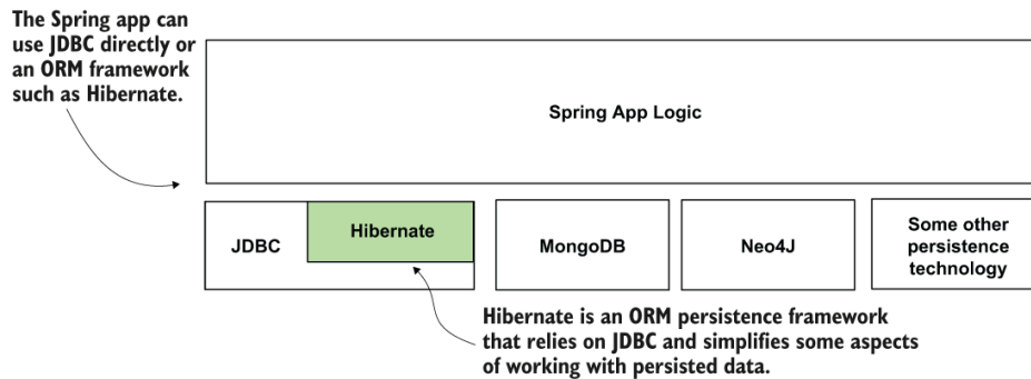
Figure 14.3 Sometimes apps use frameworks built on top of JDBC, such as Hibernate. The variety in choices makes implementing a persistence layer complex. We want to eliminate this complexity from our apps, and, as you'll learn, Spring Data helps us do this.
