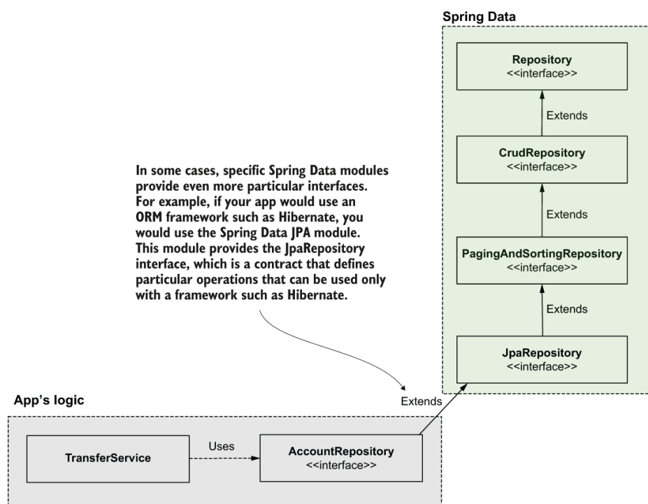
Figure 14.10 Different Spring Data modules might provide other, more particular contracts. For example, if you use an ORM framework such as Hibernate (which implements the JPA) with Spring Data, you can extend the JpaRepository interface, which is a more particular contract that provides operations applicable only when using a JPA implementation, such as Hibernate.
