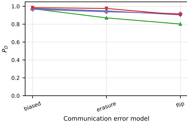
residual direct
