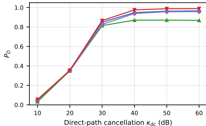
direct cancellation
