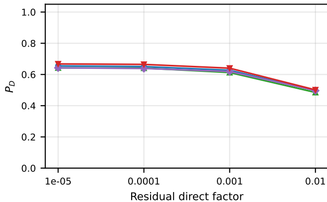
residual direct
