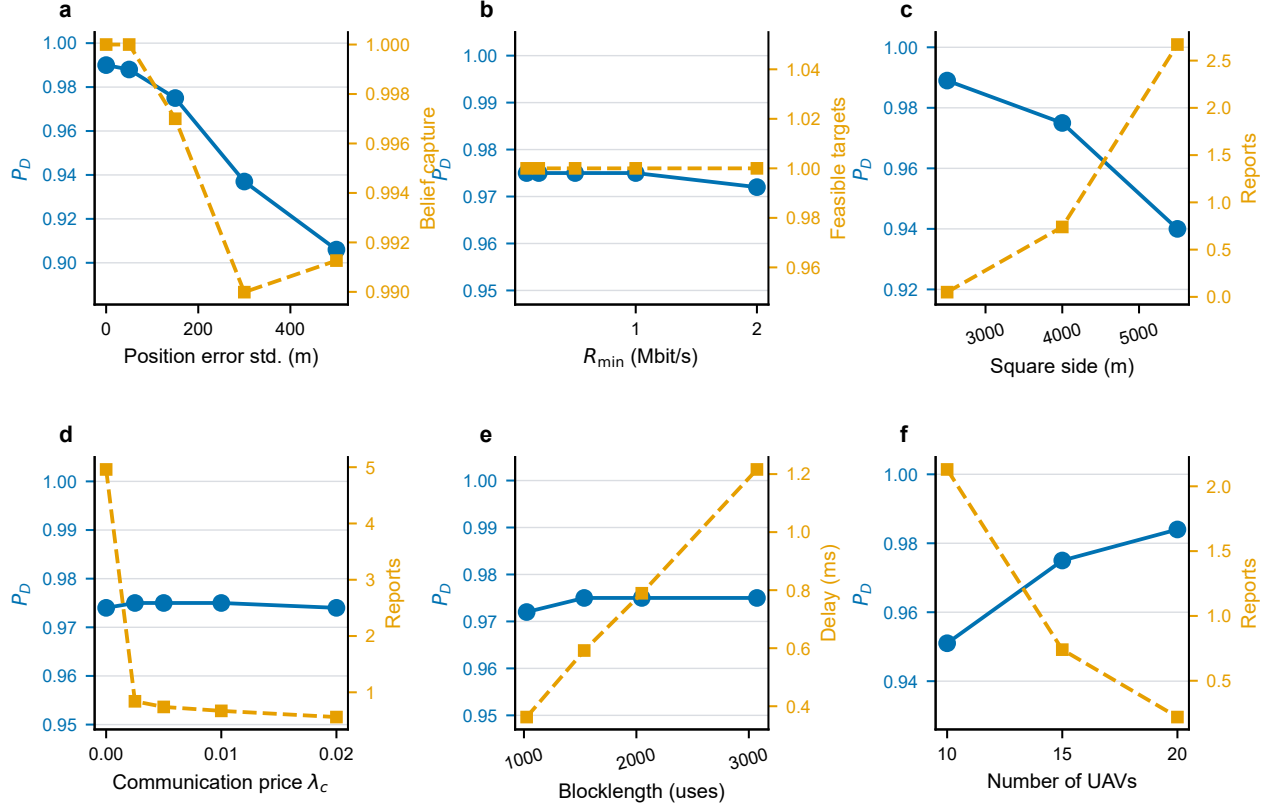
Figure 1: Operating envelope, 100 trials per condition. (a) Position-belief error, (b) minimum reporting rate, (c) deployment side, (d) communication price, (e) blocklength, (f) fleet size. Blue denotes detection probability and orange the named secondary metric. No additional uncertainty bands are shown for these diagnostic scans.
