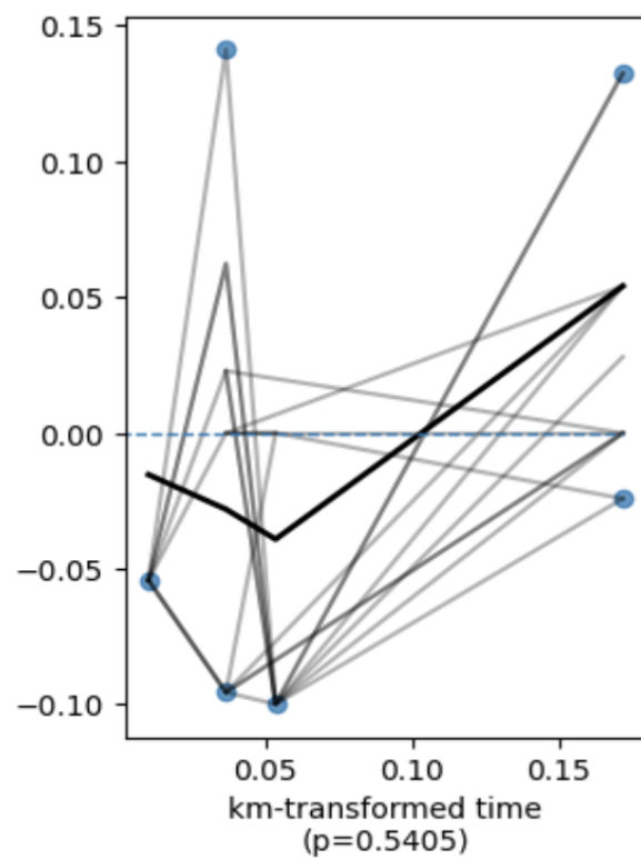
Scaled Schoenfeld residuals of 'APACHE II Score'
