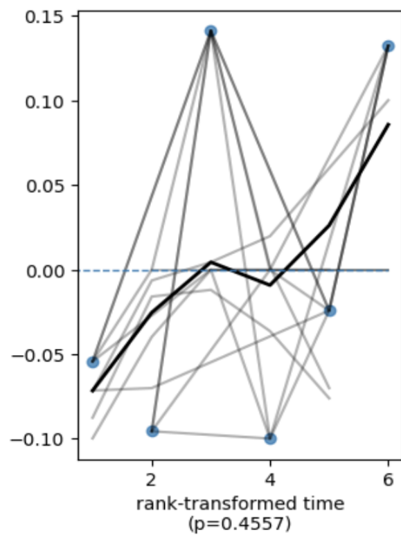
Scaled Schoenfeld residuals of 'APACHE II Score'
