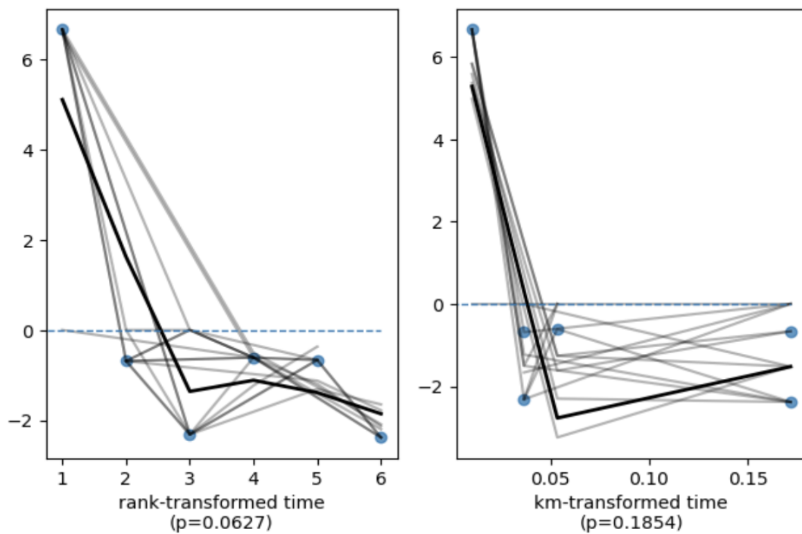
Scaled Schoenfeld residuals of 'trial_arm_num'
