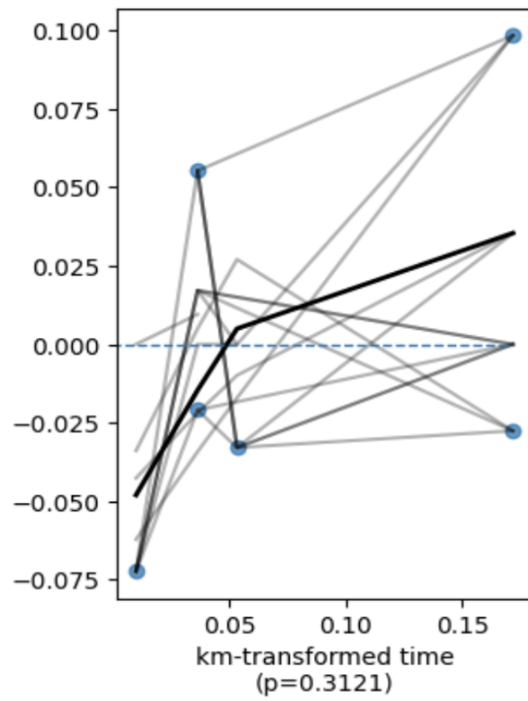
Scaled Schoenfeld residuals of 'Age'
