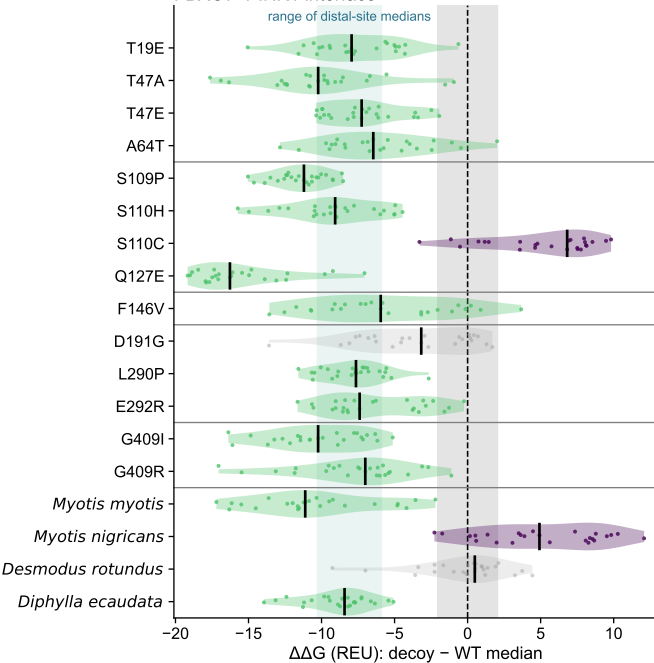
FBXO7-PINK1 interface
