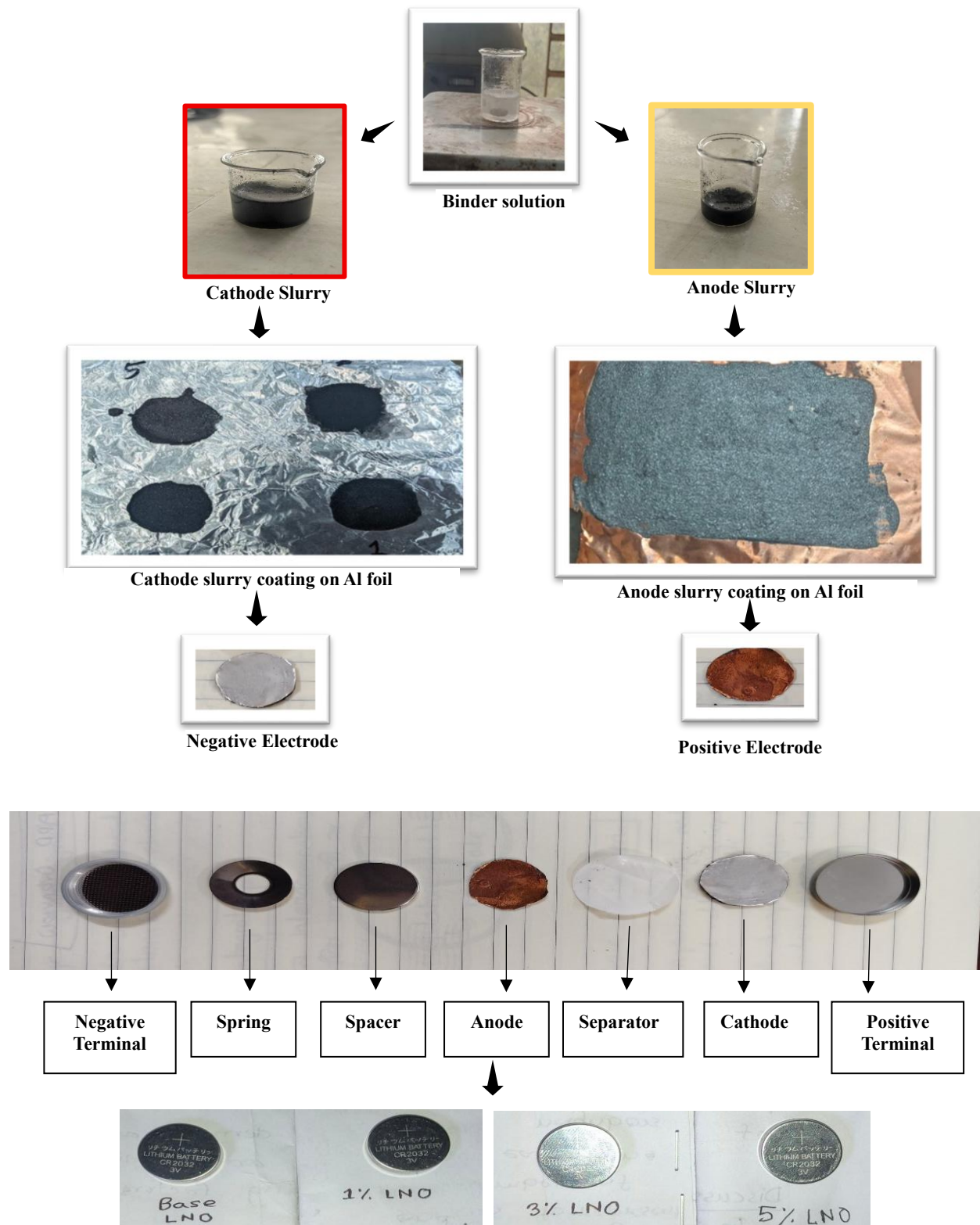
Coin Cell Assembly for Lithium-Ion Battery
