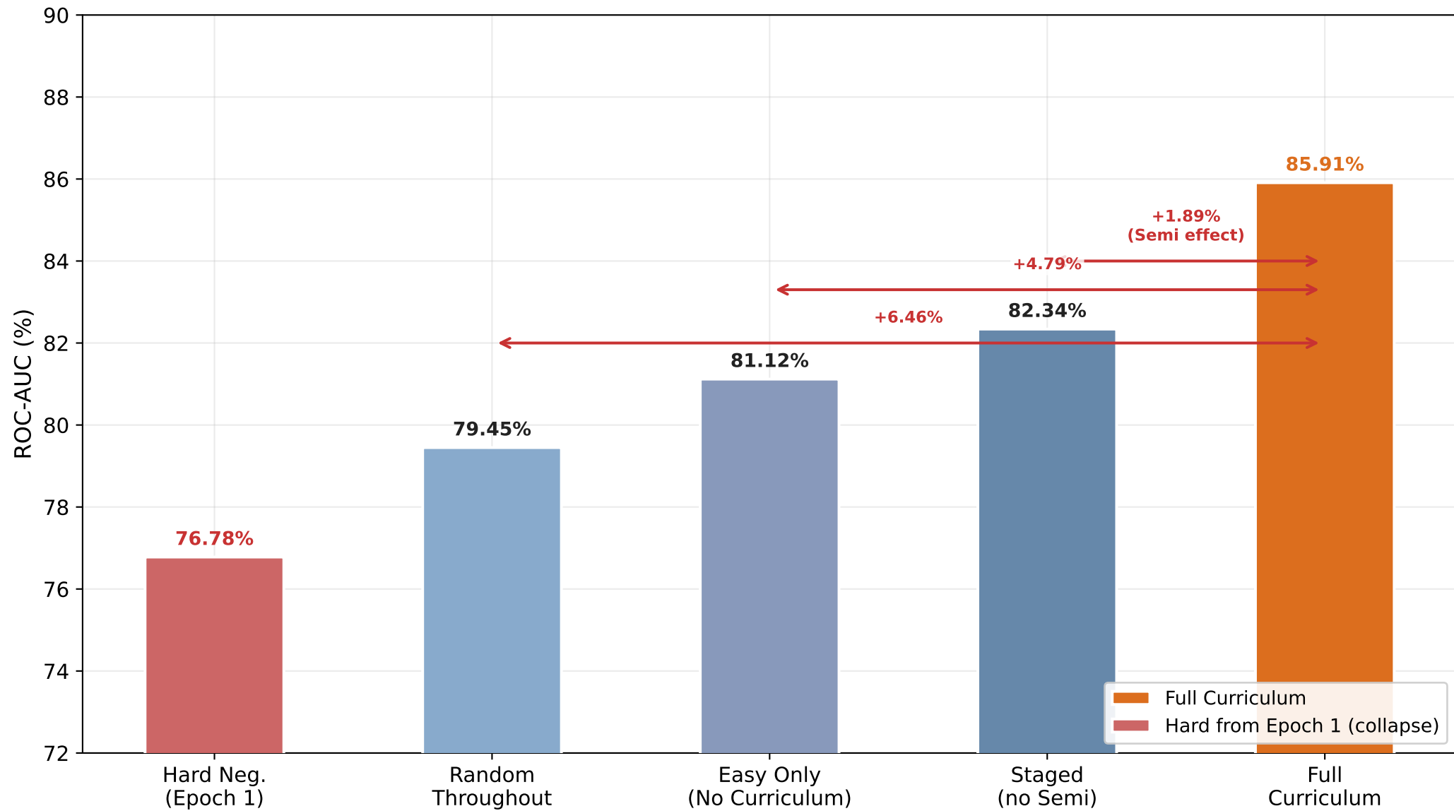
Curriculum Schedule Ablation (Amazon)
