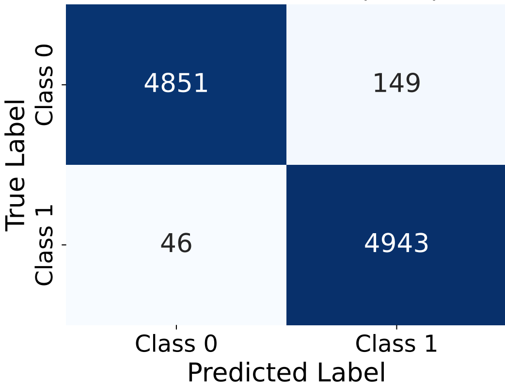
Confusion Matrix (Train)
