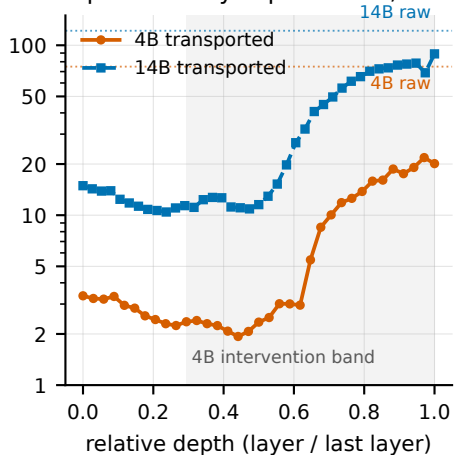
B. Collapse severity is per-model, not depth
