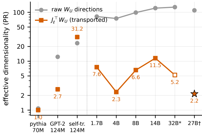
A. Transport collapses directional diversity
