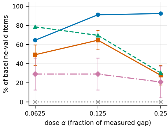
Qwen3-4B (n = 79, covert n = 24)
