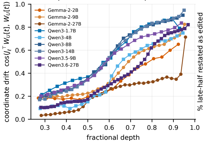
Swap direction drifts to output coords
