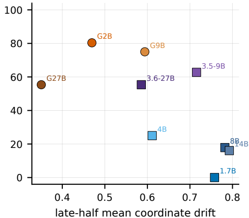
Drift orders late-band capture, coarsely
