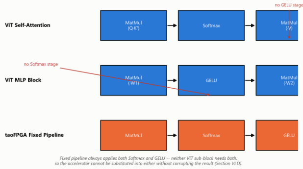
Fig. 9. Real ViT self-attention and MLP dataflows contrasted with taoFPGA's fixed fused pipeline.
