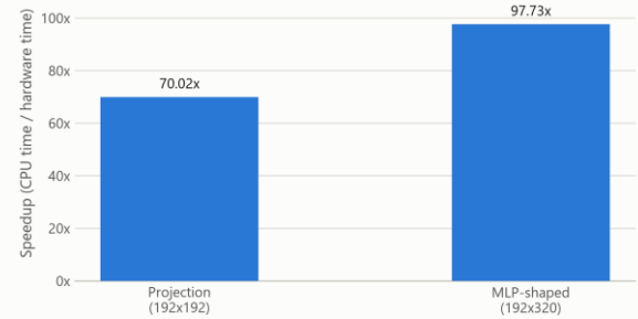
Fig. 8. Measured hardware kernel speedup over CPU.
