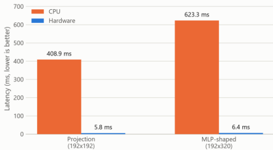
Fig. 6. Latency, CPU vs. hardware, both benchmarked shapes.
