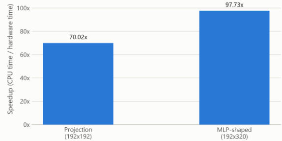
Fig. 3. Measured hardware kernel speedup over CPU.
