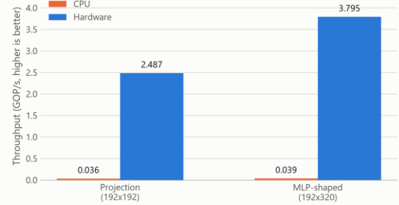
Fig. 2. Throughput (GOP/s), CPU vs. hardware, both shapes.
