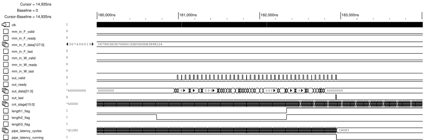
Figure A.2: Cadence SimVision detailed timing trace capturing the end-of-inference sequence ( \sim 180\mu s to \sim 183.5\mu s ). The trace details output stream handshaking ( out_valid , out_data[31:0] ), end-of-packet demarcation (a single-cycle out_last pulse), Softmax phase progression ( length1_flag , length2_flag ), and the pipeline latency counter converging precisely at 18,083 cycles.
