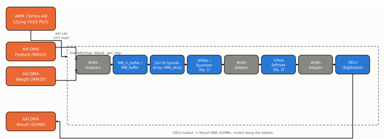
Fig. 3. Complete top-level SoC architecture: PS7, three AXI DMA channels, and the transformer_block_axi_top internal pipeline.
