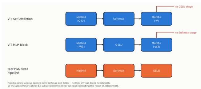
Fig. 9. Real ViT self-attention and MLP dataflows contrasted with taoFPGA's fixed fused pipeline.
