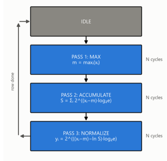
Fig. 2. Softmax_control's 3-pass FSM and its per-pass equations (Eq. 2).
