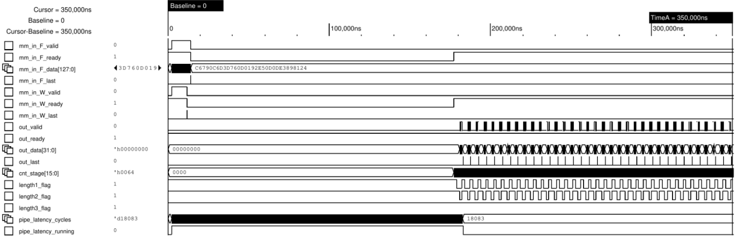
Figure A.1: Cadence SimVision full-pipeline simulation trace ( transformer_block_tb ). The waveform captures end-to-end execution across \sim 350\mu s : initial weight and activation ingestion over AXI-Stream interfaces ( mm_in_W_valid , mm_in_F_valid ), three-pass Softmax execution flags ( length1_flag , length2_flag , length3_flag ), and continuous streaming output, confirming the measured latency of 18,083 clock cycles.
