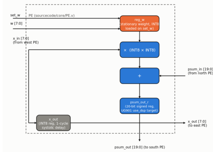
Fig. 1. One PE's internal datapath: stationary weight register, INT8 multiply, 20-bit accumulate, and systolic x/psum propagation.
