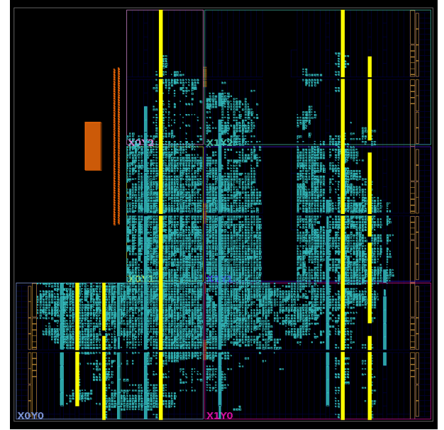
Fig. 5. Vivado Device view (post-implementation): physical cell placement across the Zynq-7020 fabric, with column-structured DSP/BRAM resources (yellow) and clock-region boundaries (X0Y0-X1Y2).
