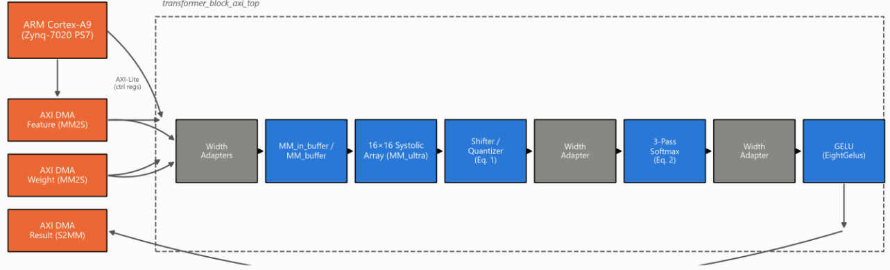
Fig. Y. Top-level SoC datapath: PS7, three AXI DMA channels, and the transformer_block_axi_top accelerator pipeline.
