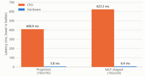
Fig. 1. Latency, CPU vs. hardware, both benchmarked shapes.
