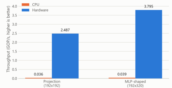
Fig. 2. Throughput (GOP/s), CPU vs. hardware, both shapes.
