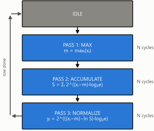
Fig. X. Softmax_control's 3-pass FSM: each pass streams the full N-element row once, serially -- total latency 3N cycles.
