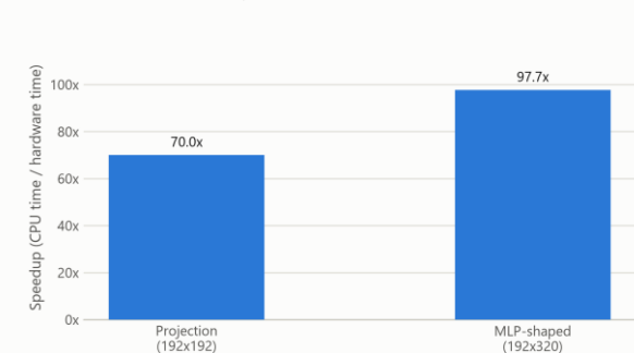
Hardware Kernel Speedup Same fused matmul+softmax+GELU operation, hardware vs. CPU
