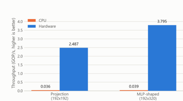
Throughput: CPU vs. Hardware Accelerator ViT-Tiny-representative matmul+softmax+GELU kernel
