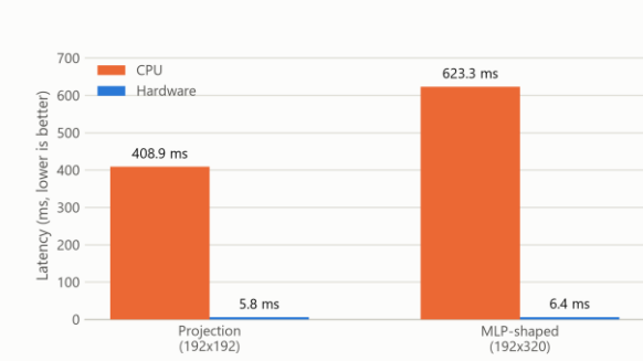
Latency: CPU vs. Hardware Accelerator ViT-Tiny-representative matmul+softmax+GELU kernel
