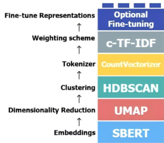
Fig. 2. Modular architecture of the BERTopic pipeline.
