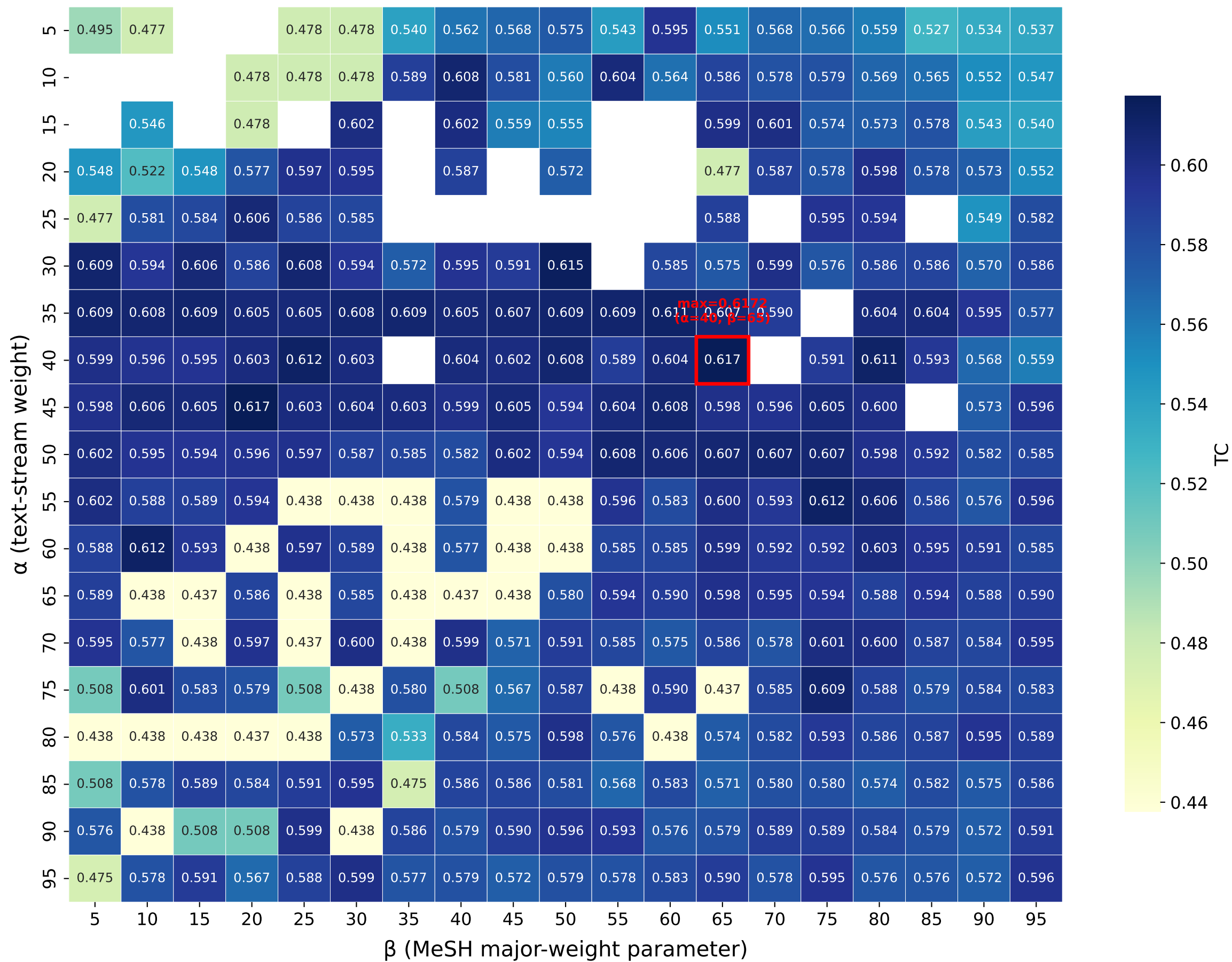
Topic Coherence (TC) — Dual PubMedBERT, Full Text
