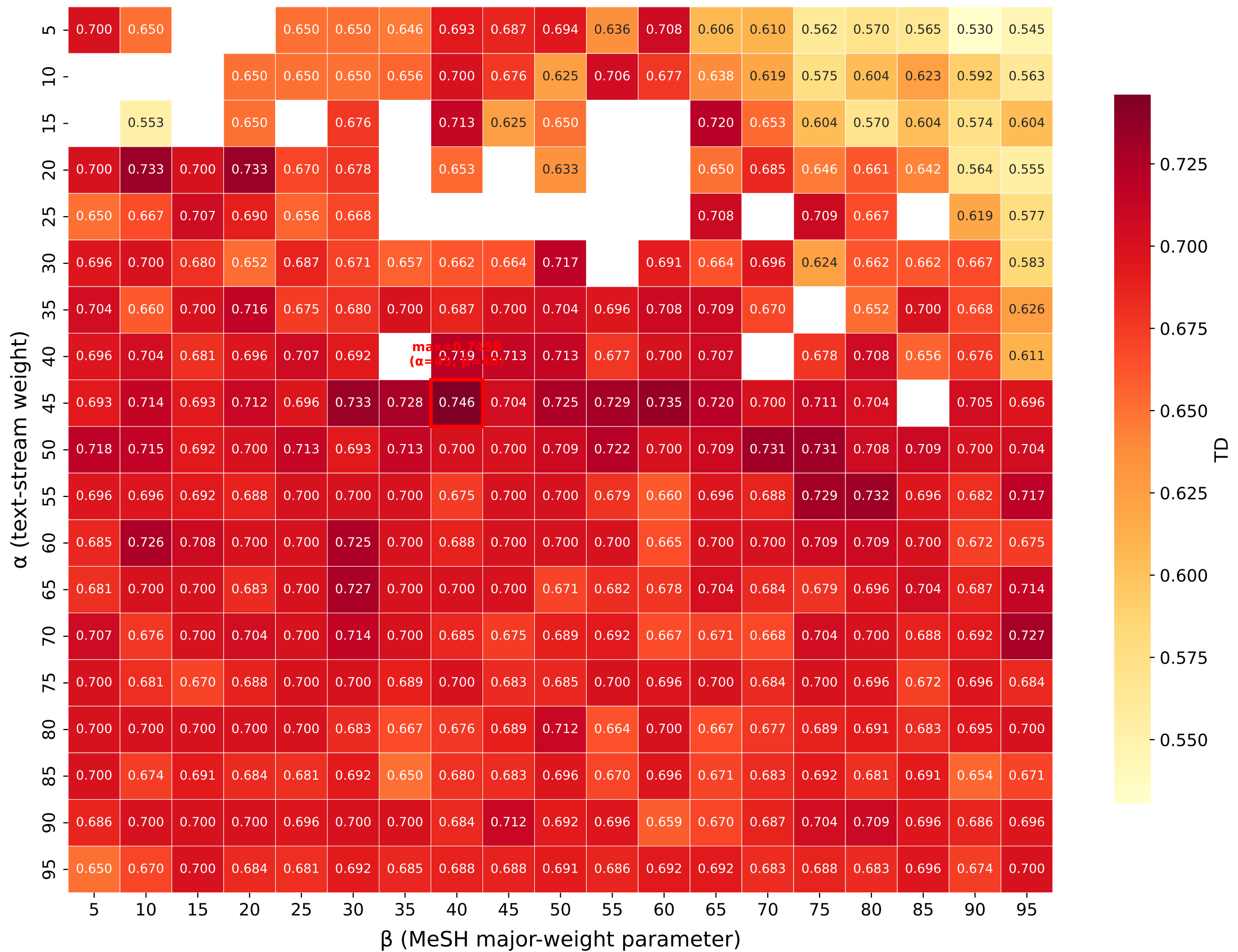
Topic Diversity (TD) — Dual PubMedBERT, Full Text
