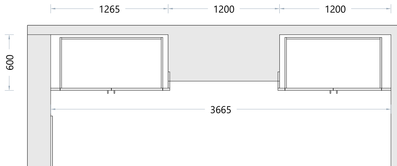
TOP VIEW 1:25@A3
