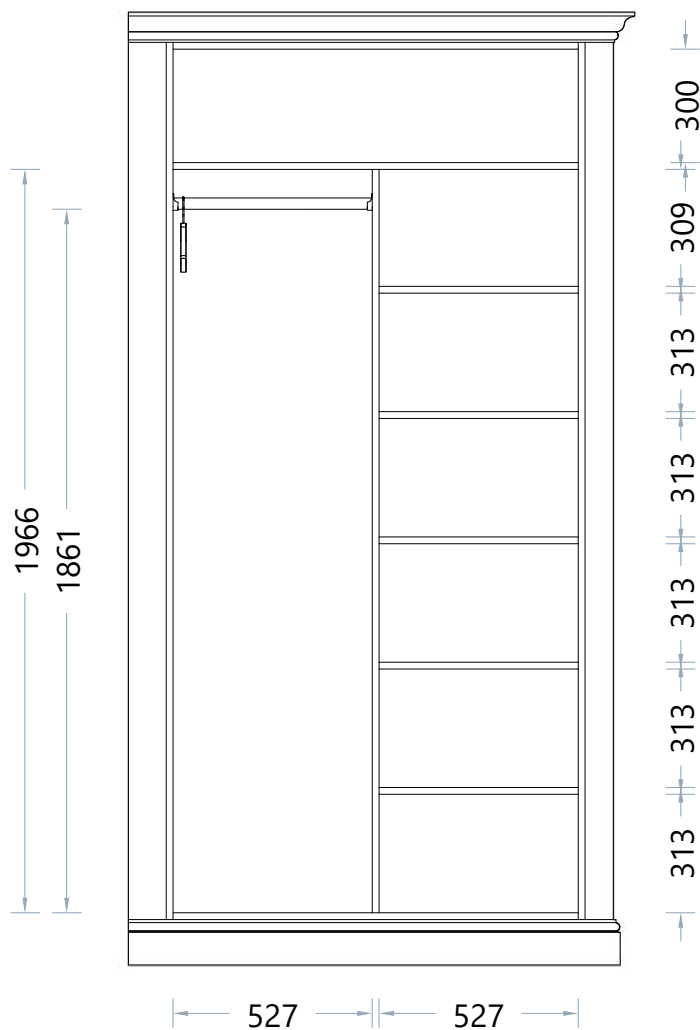
FRONT VIEW 1:25@A3
