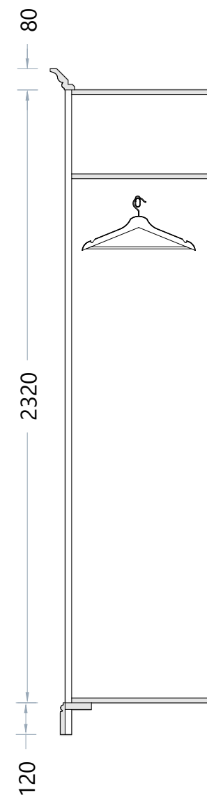
SECTION THROUGH LH UNIT 1:25@A3
