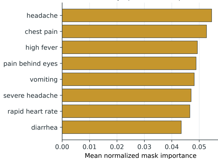
Oracle TabNet symptom-mask importance
