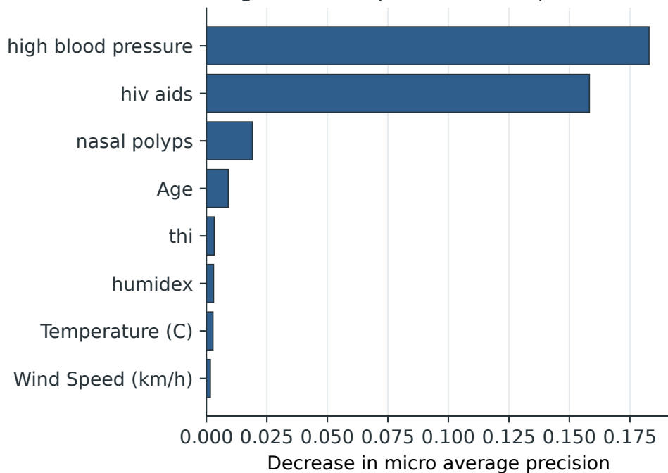
Stage-1 context permutation importance
