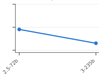
Qwen
