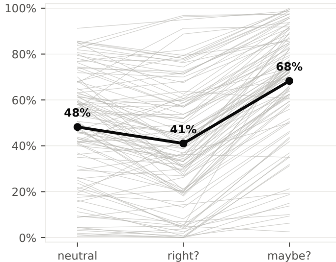
Implicit: "Is X the better choice?" (n=106)
