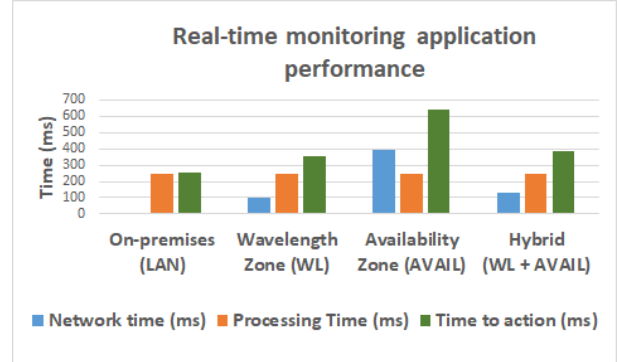
Fig. 9: Real-time monitoring application performance
