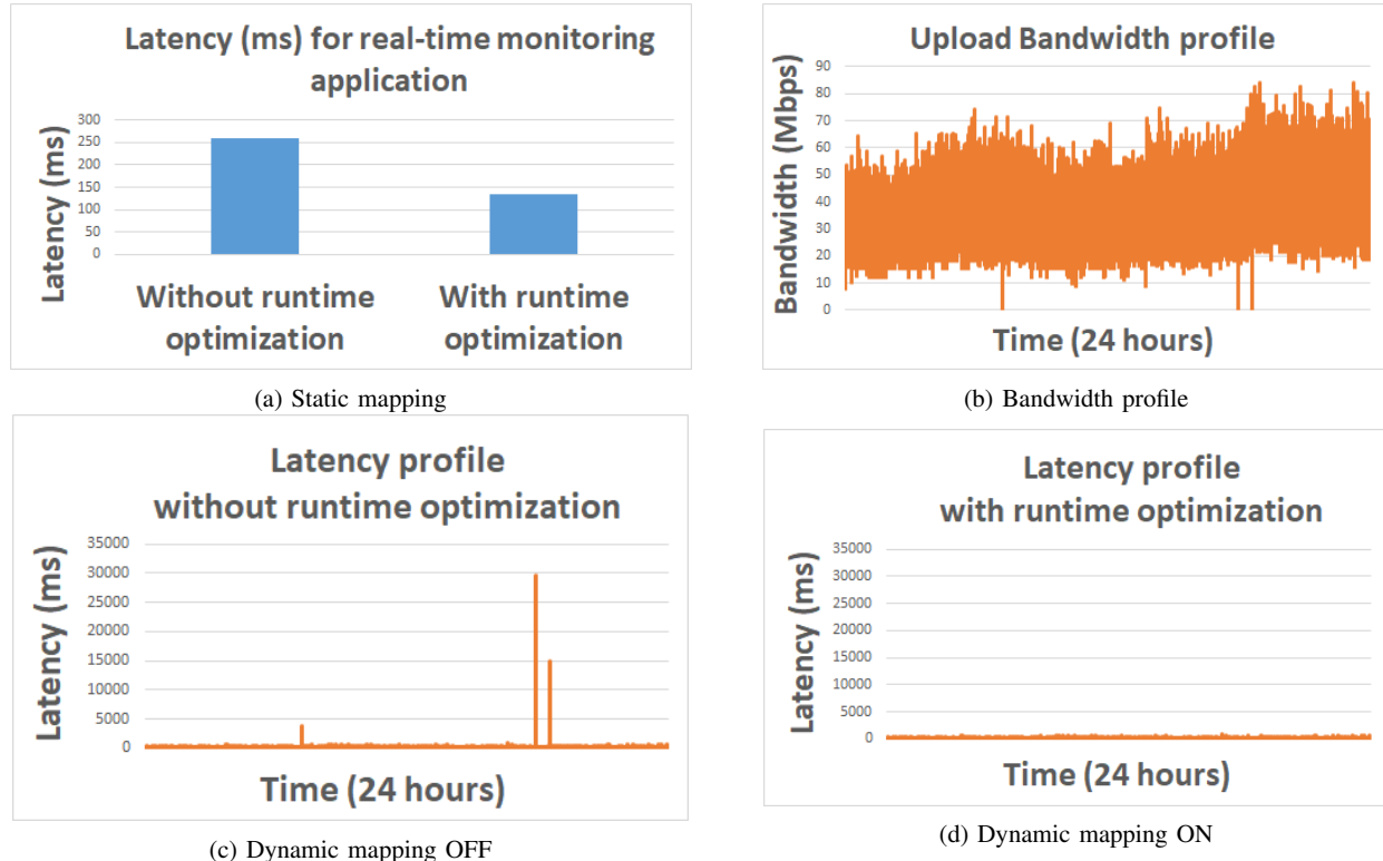
Fig. 11: Impact on latency
