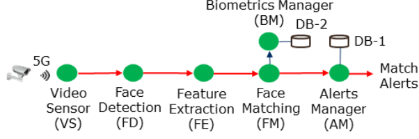
Fig. 3: Real-time monitoring application pipeline
