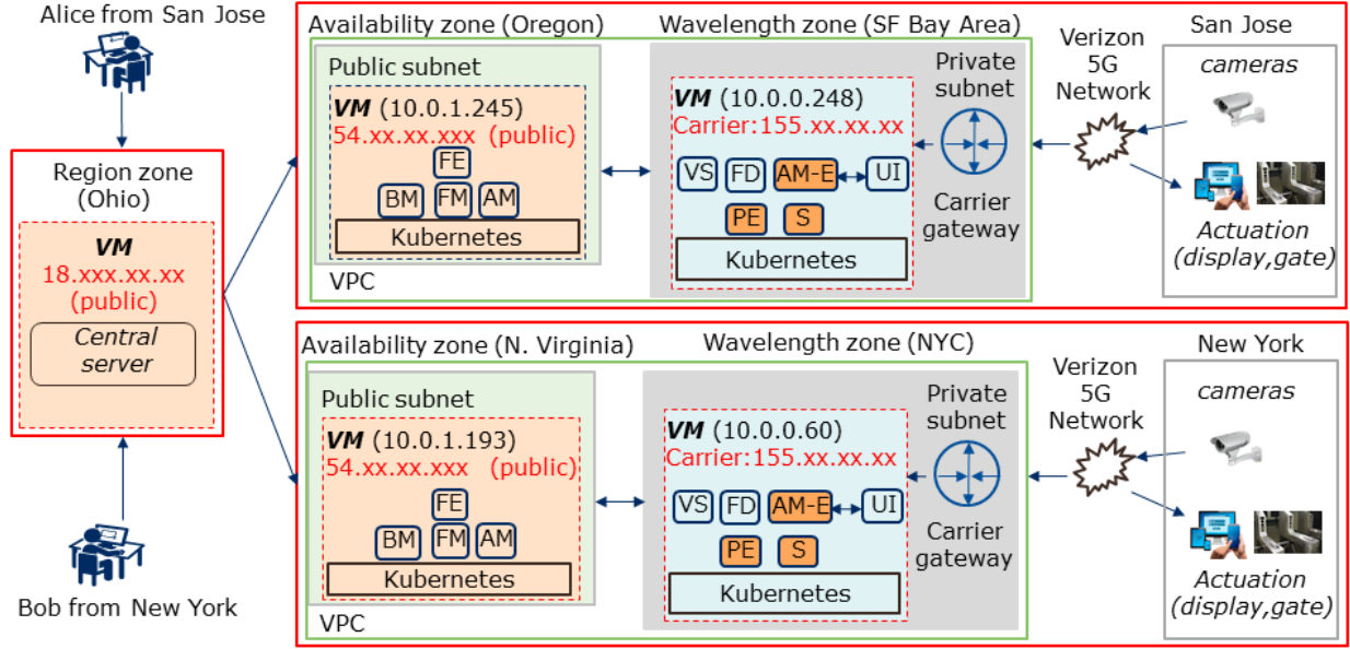
Fig. 6: Test bed for 5G applications in edge-cloud
