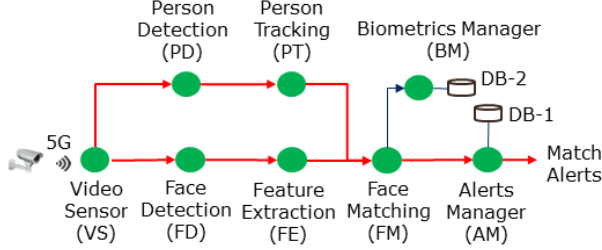
Fig. 4: Application pipeline for variant of real-time monitoring
