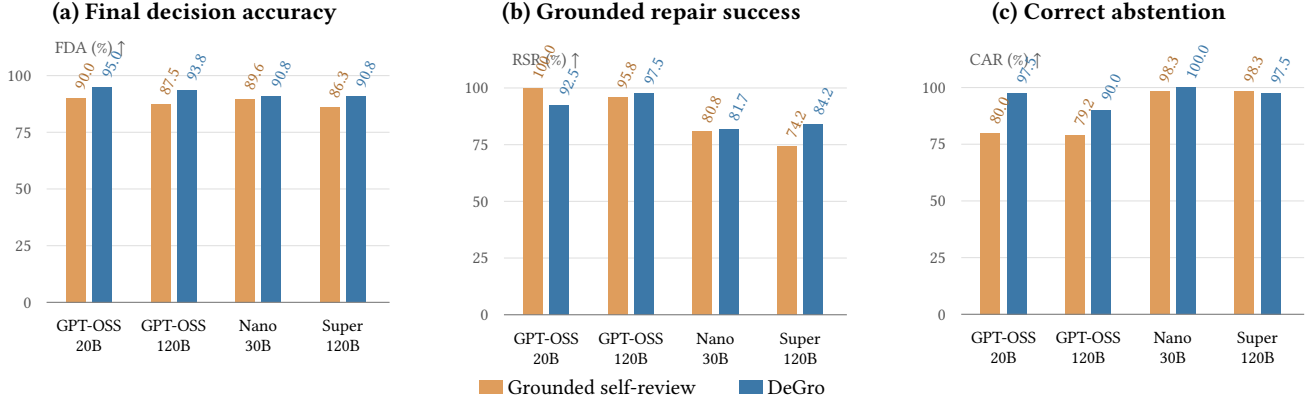
Figure 3: Main-experiment comparison on the same fixed 120 pairs. DeGro has higher FDA than grounded self-review for all four models, while RSR and CAR expose model-specific tradeoffs. The GPT-OSS 20B comparison is preregistered; the other models are post-hoc, and both Nemotron FDA differences are statistically inconclusive. All axes start at zero.
