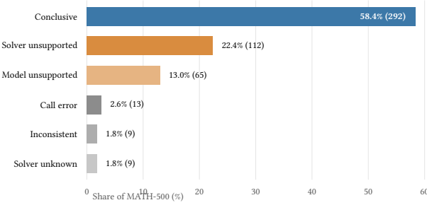
Figure 6: Frozen MATH-500 cohort accounting for all 500 shared initial structured specifications. Solver-level unsupported cases are the largest exclusion category.
