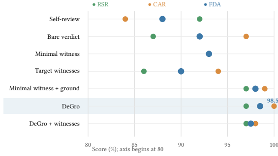
Figure 4: Exploratory GPT-OSS 20B ablation on 100 development pairs. Concrete witnesses do not improve FDA over DeGro without witnesses. ORR is omitted because it is exactly 100 – CAR.
