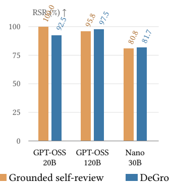
Figure 3: MIRA-Math comparison on the same fixed 120 pairs. DeGro has higher FDA than grounded self-review for all three models, while RSR and CAR expose model-specific tradeoffs. The GPT-OSS 20B comparison is preregistered; the GPT-OSS 120B and Nemotron Nano comparisons are post-hoc, and the Nano FDA difference is statistically inconclusive. All axes start at zero.
