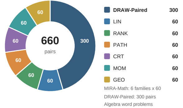
Figure 3: Paired benchmark composition. DRAW-Paired contributes 300 pairs constructed from natural algebra word-problem sources; MIRA-Math contributes six 60-pair families: linear separation (LIN), rank-deficient systems (RANK), path sums (PATH), Chinese-remainder reconstruction (CRT), moment constraints (MOM), and geometry (GEO). Every pair yields one OMISSION and one UNDERSPECIFIED case.
