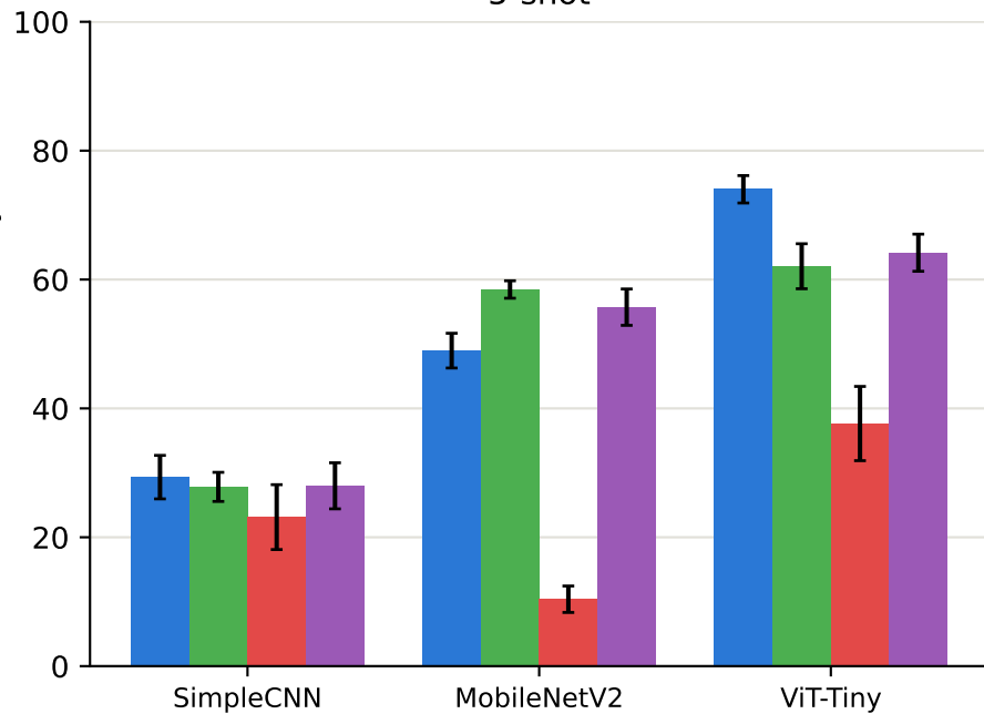
5-shot
