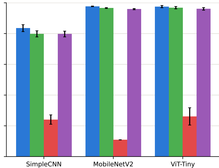
Full data
