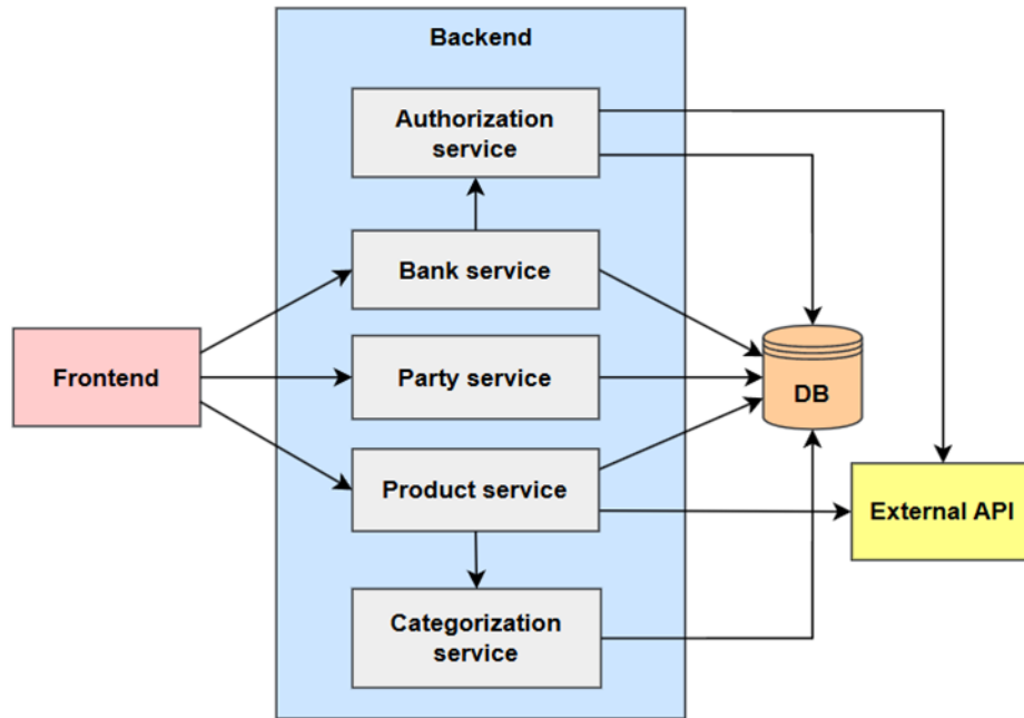
Figure 4.1. Application Architecture
