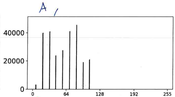
ORIGINAL HISTOGRAM
