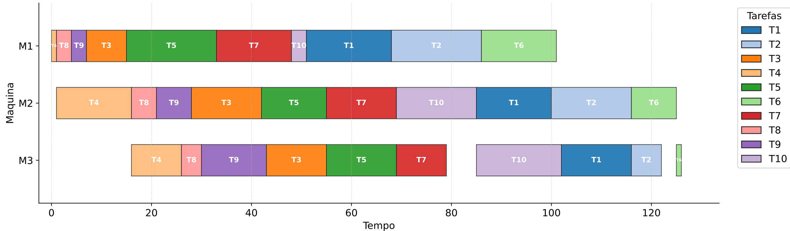
Flow Shop Scheduling - problem_3m_10j - makespan = 126.000
