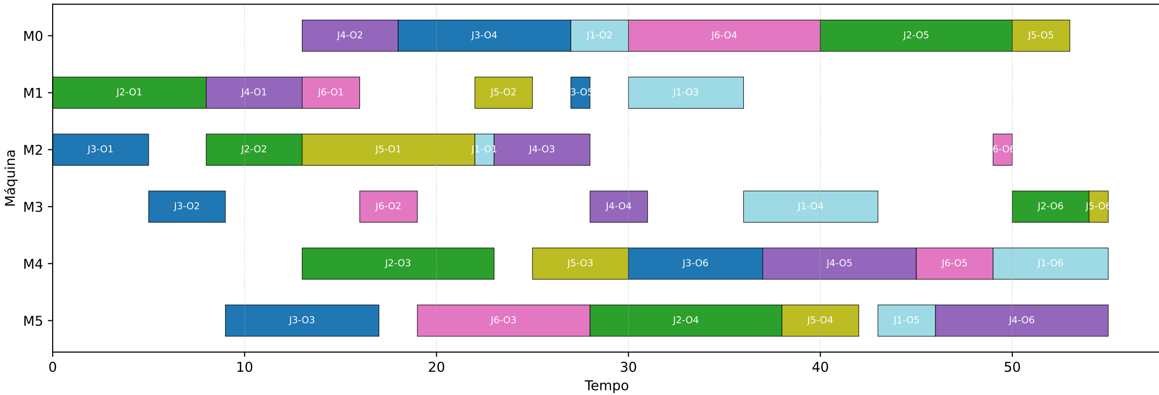
Job Shop Scheduling - ft06 - makespan = 55.000
