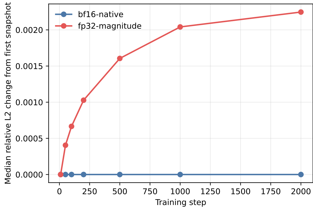
Raw QDoRA magnitude movement across saved checkpoints
