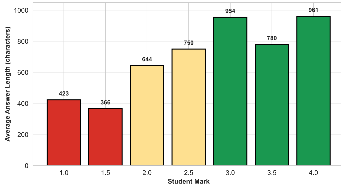
Answer Length vs Marks Received
