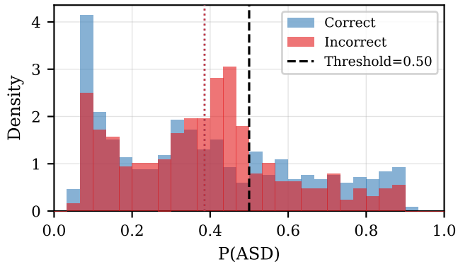
Confidence by Correctness
