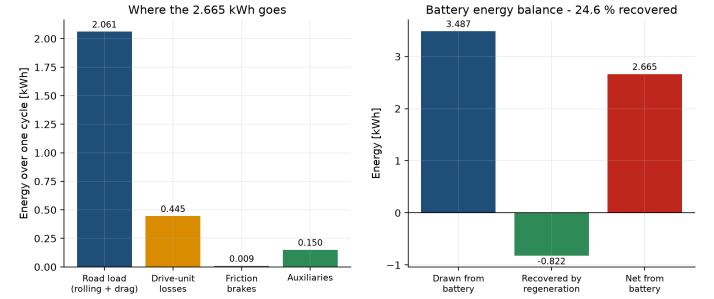
Figure 9: Energy expenditure over one cycle and the battery energy balance, showing the share recovered by regeneration.
