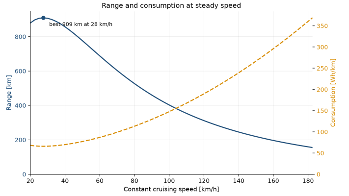
Figure 11: Range and consumption at steady cruising speed. The interior maximum arises from the competition between the constant auxiliary load and aerodynamic drag.
