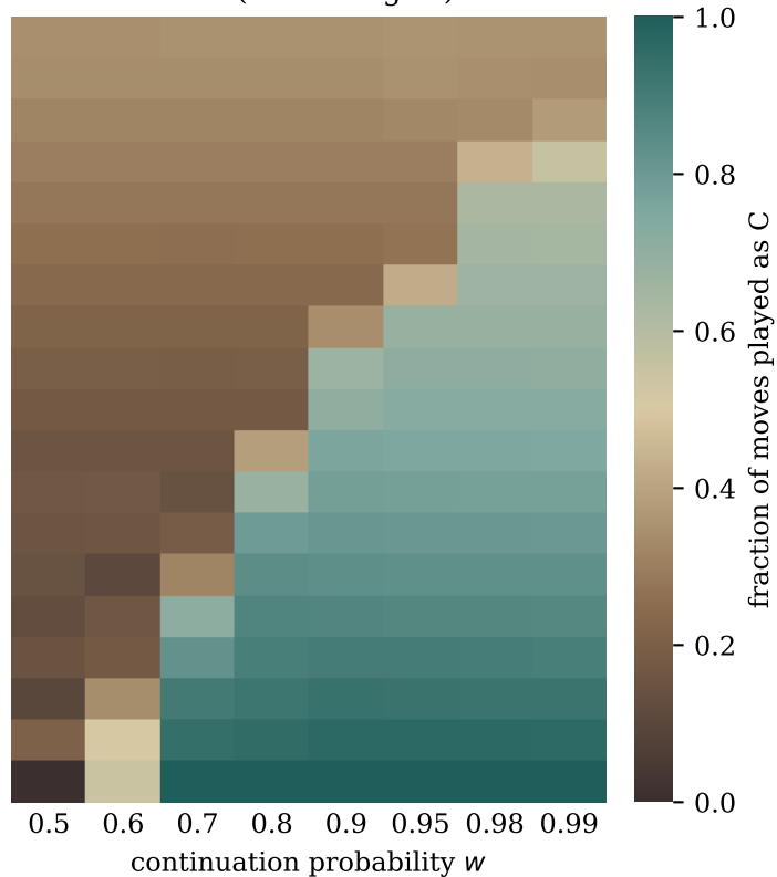
Pool (15 strategies)
