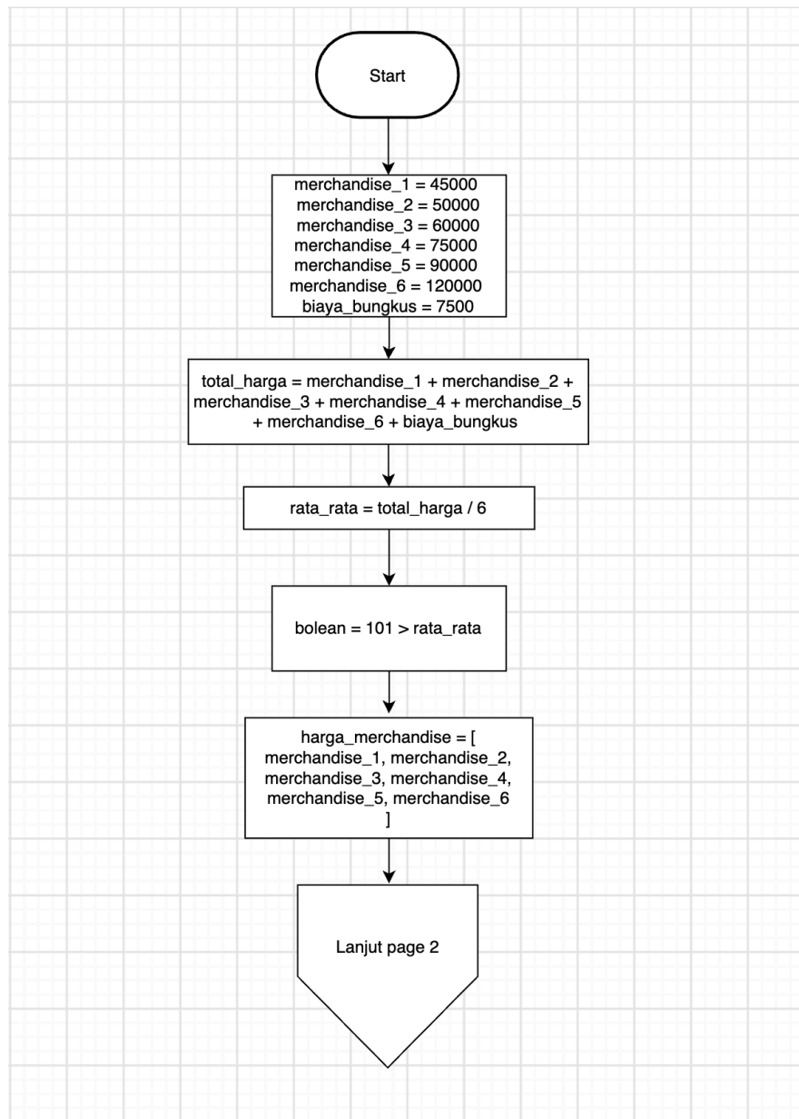
Gambar 1.1 Flowchart
