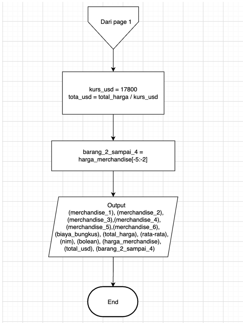
Gambar 1.2 Flowchart
