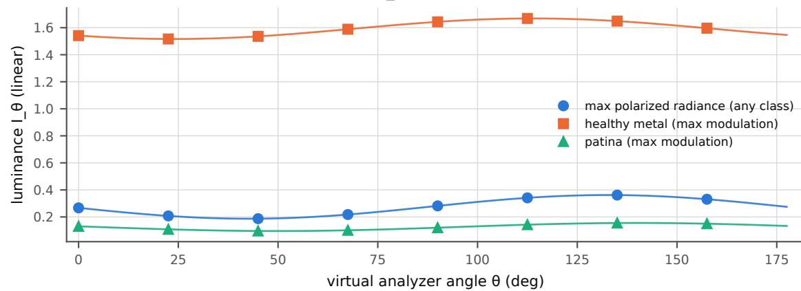
Analyzer response of three pixels: I_\theta = \frac{1}{2}(S_0 + S_1 \cos 2\theta + S_2 \sin 2\theta) , period 180^\circ
