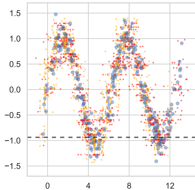
h = 0.03
