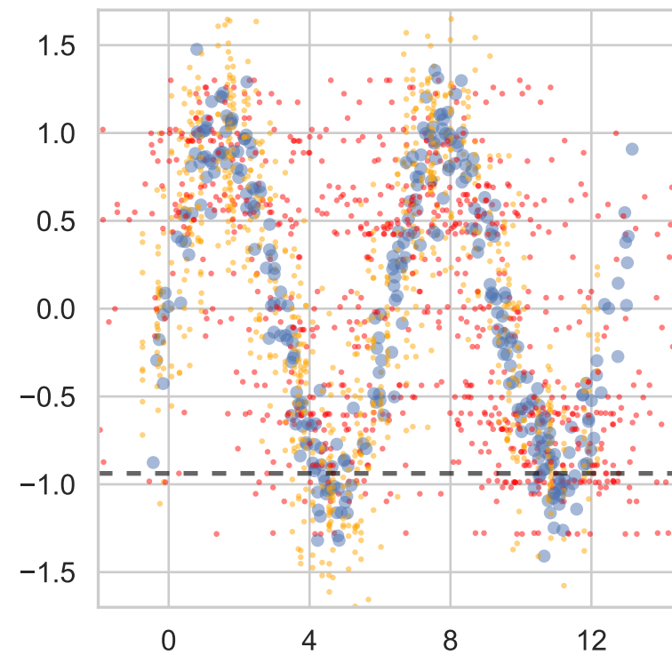
h = 0.1
