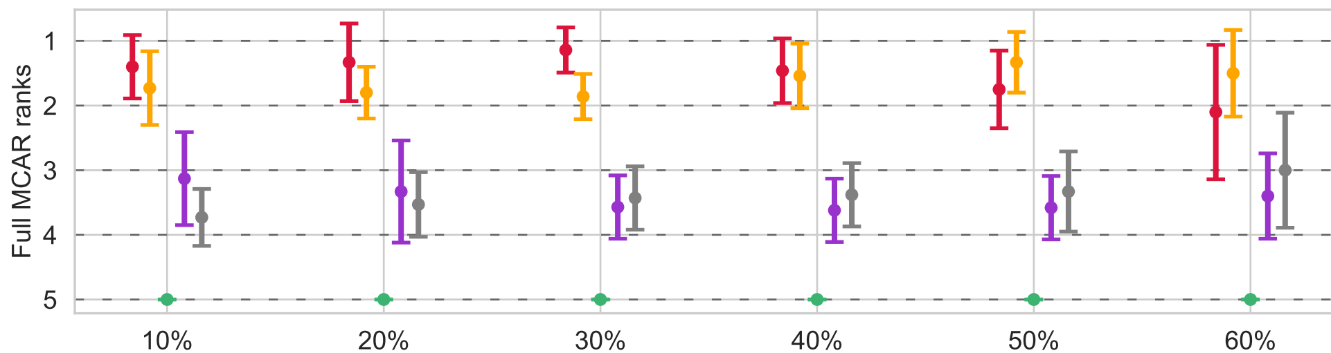
Log-likelihood rankings
