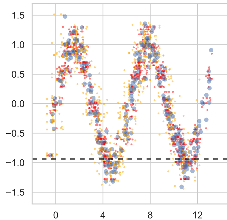
h = 0.01
