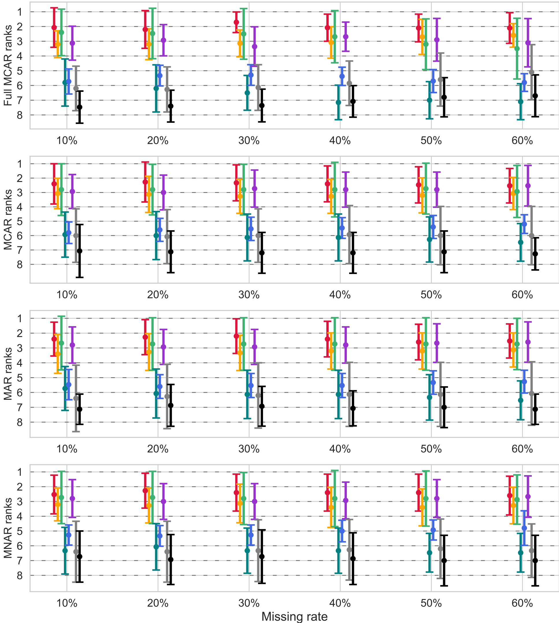
NRMSE rankings
