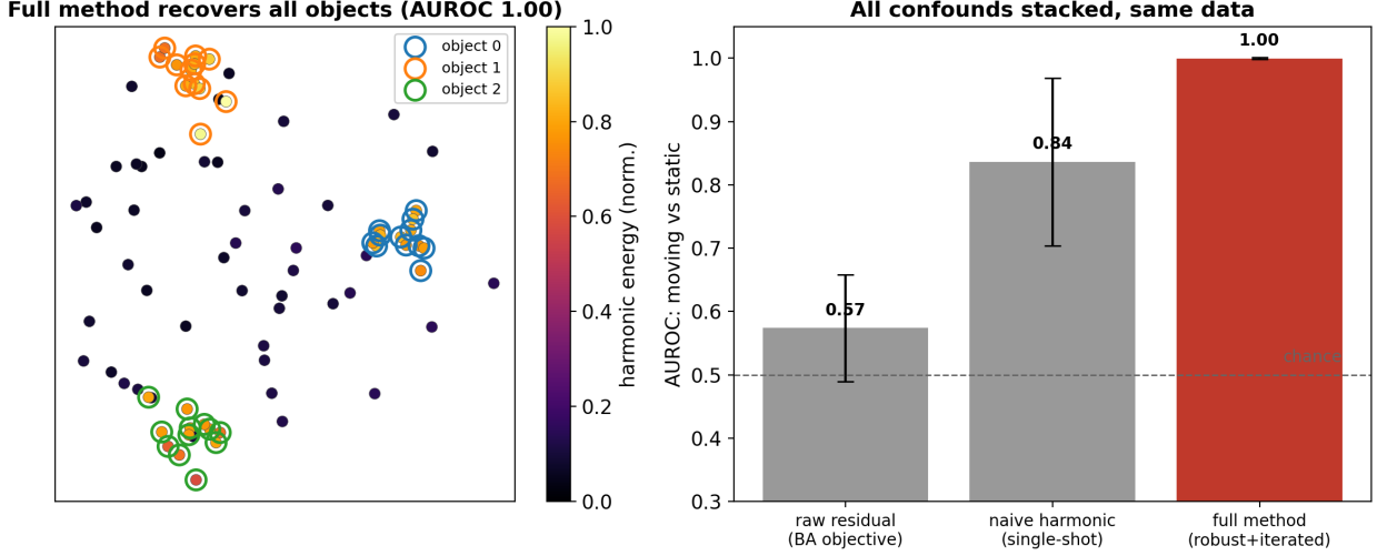
Figure 3: All boundaries stressed at once. A scene with three moving objects, static fraction 0.56, accumulating camera drift (0.45 rad/step), and per-view Sim(3) scale ambiguity. Left : harmonic energy from the full solver, concentrated on all three objects (colored rings; AUROC 1.00). Right : localization AUROC on the same data under three readings (mean \pm s.d., 6 seeds): the bundle-adjustment residual is at chance, a naive single solve is degraded and high-variance, and the full robust, iterated, scale-anchored method is near-perfect.
