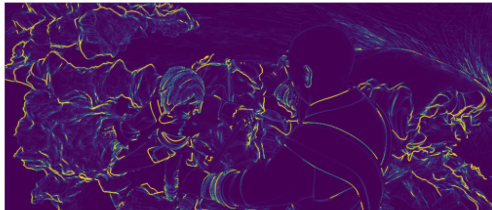
weight w_i = 1 + \gamma \min(|K_i|/\bar{S}, \tau)
