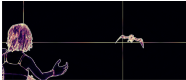
|K_i| (curvature)
