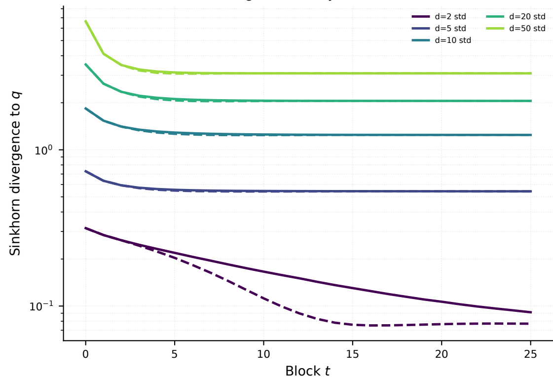
E9 dimension scaling — flatvalley (solid=std, dashed=acc)
