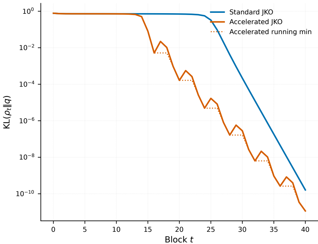
double-well ( \lambda < 0 ), init \mathcal{N}(0.5, 2.0^2)
