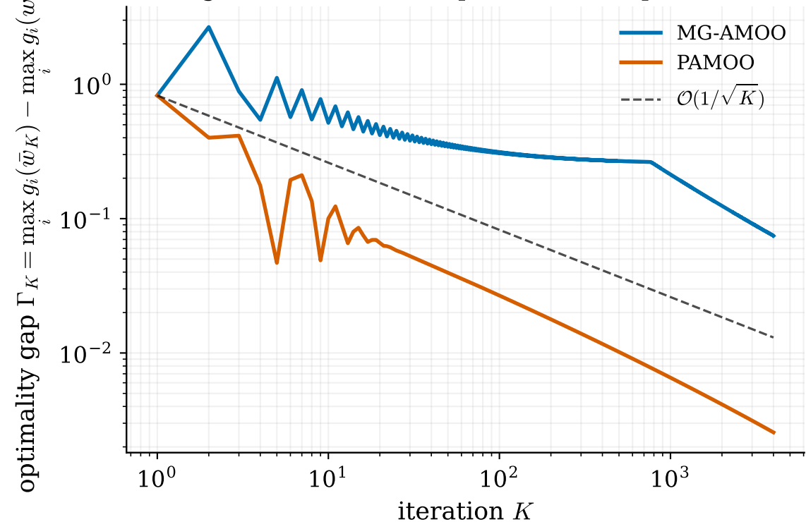
Convergence to the SOCP optimum at the predicted rate
