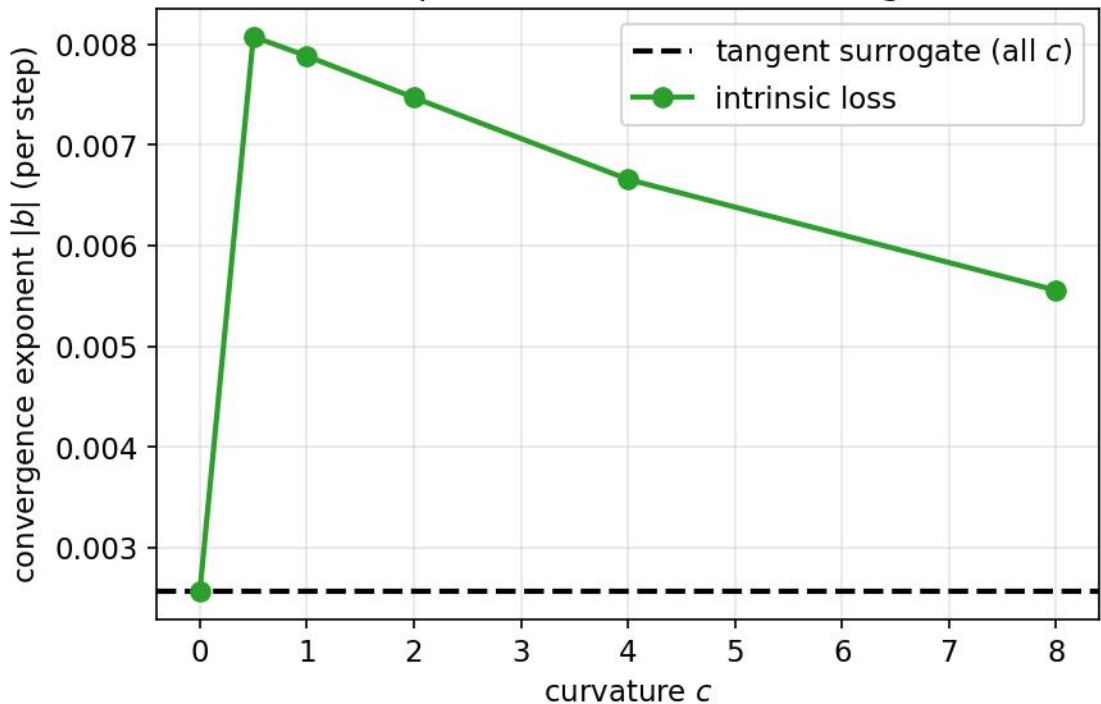
Curvature collapse check: intrinsic \rightarrow tangent as c \rightarrow 0
