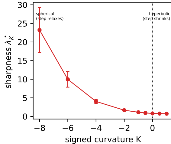
(b) landscape sharpness at optimum
